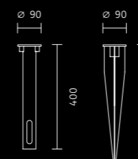
Erdanker und Erdspeiß / Ground anchor and ground spike
